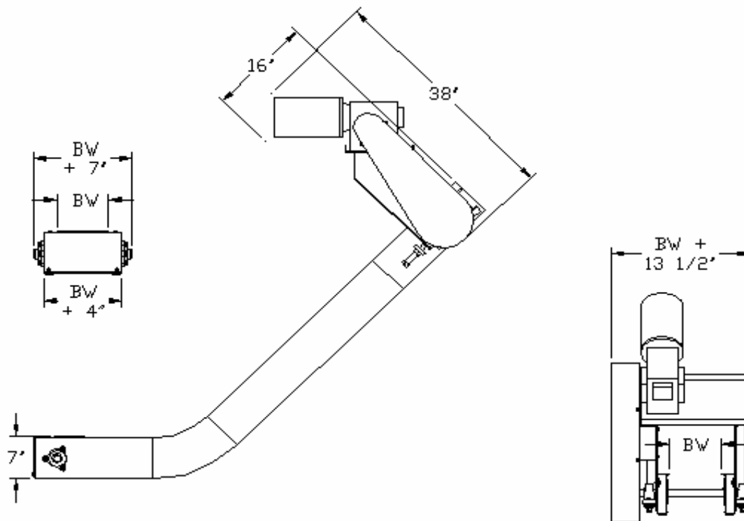
45° TOP MOUNT DRIVE
